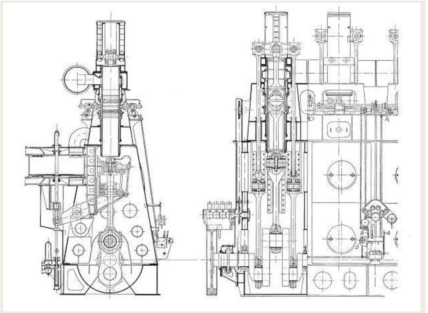
SFJ00319500160001 MT VESTFOLD. Doxford hovedmotor
